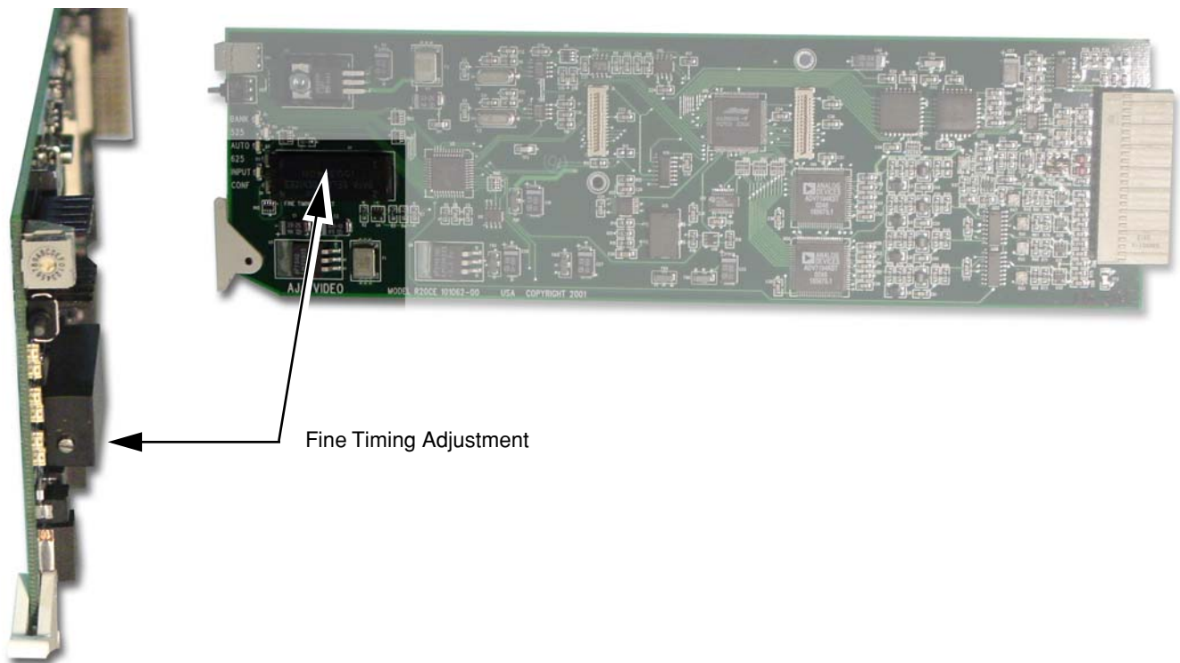
R20CE Fine Timing Adjustment Control Location
